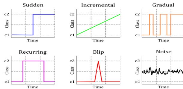
Fig. 1. Different types of Concept Drifts
