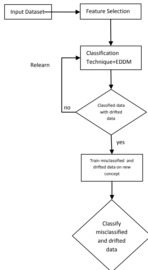
Figure 3. Work Flow of proposed plan
