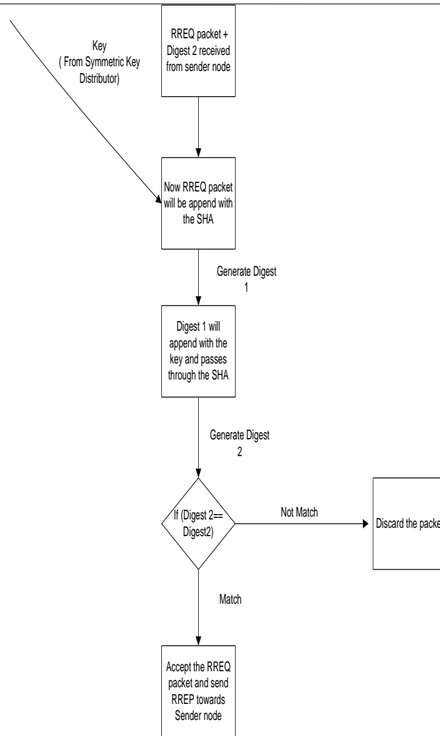
Fig.3 Destination node algorithm.
