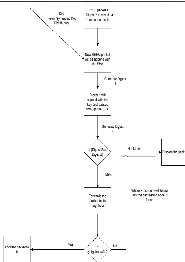
Fig.2 Intermediate node algorithm.
