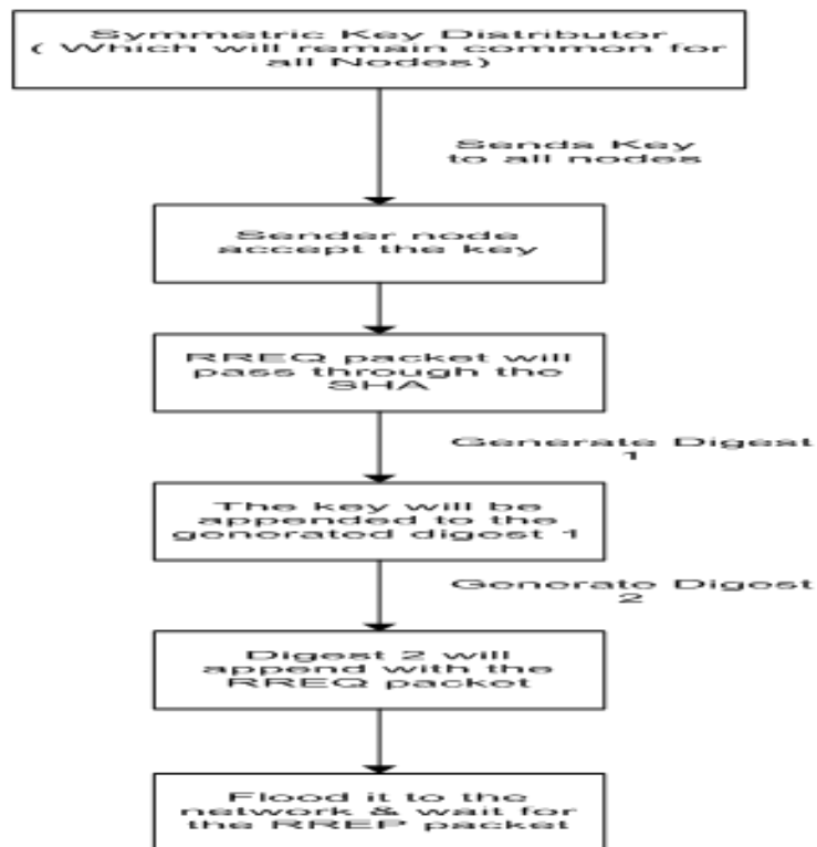
Fig.1 Sender node algorithm.
